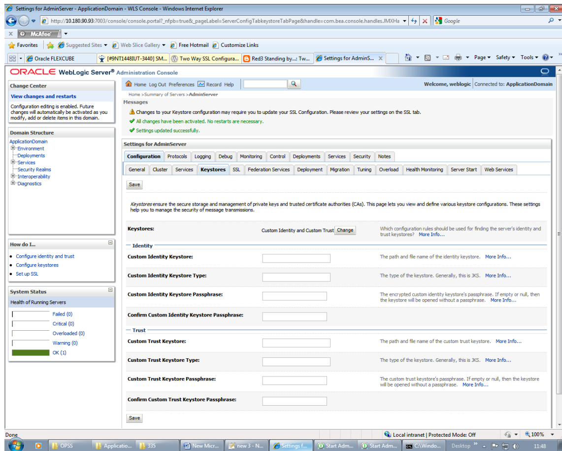
Figure 3–6 Keystores - Identity and Trust
