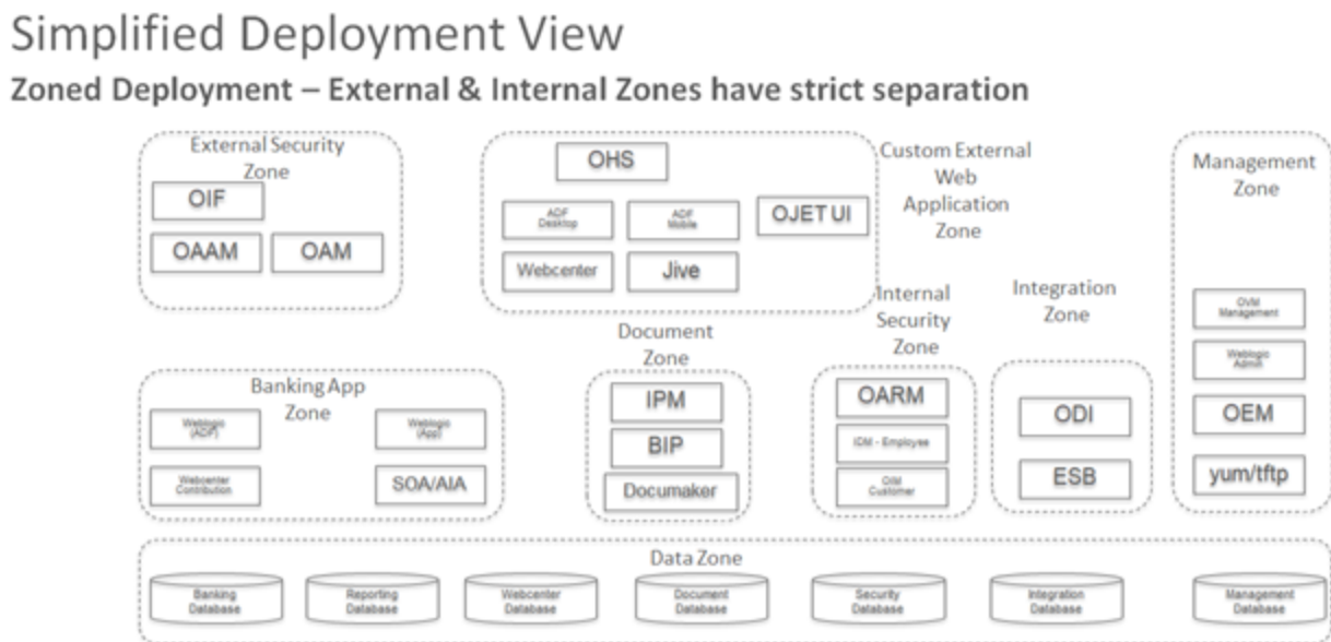
Figure 3–1 Simplified Deployment View
